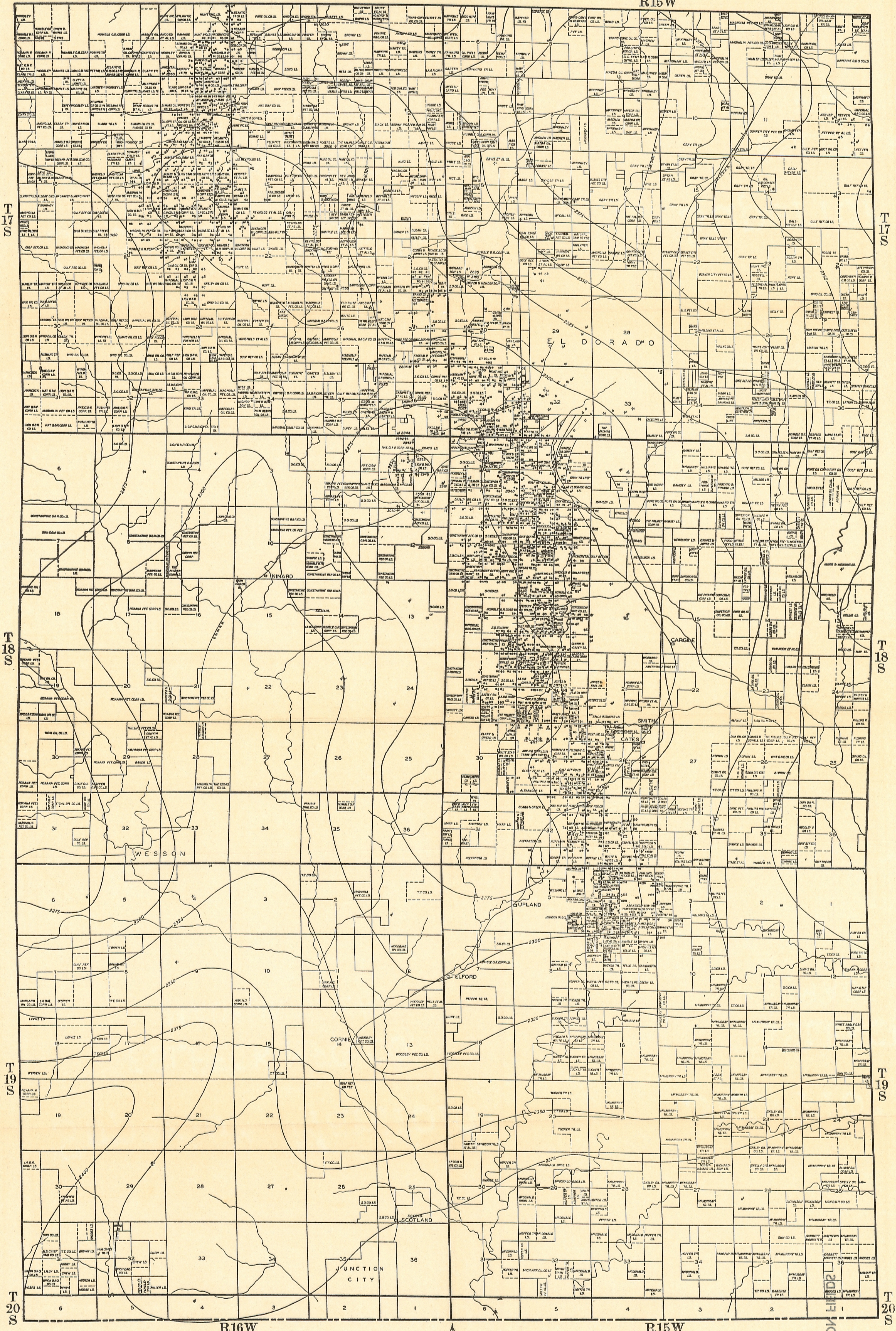
EL DORADO AND LISBON FIELDS STRUCTURE CONTOURS DRAWN ON TOP OF MEAKIN SAND CONTOUR INTERVAL 25 FEET - FIGURES GIVE DEPTHS BELOW SEA LEVEL SCALE 0 1000 2 3 4 5 6 7 8000
